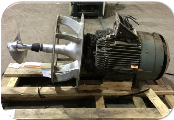
Aqua-Jet® Aerator Power Section Prior to Rebuild
